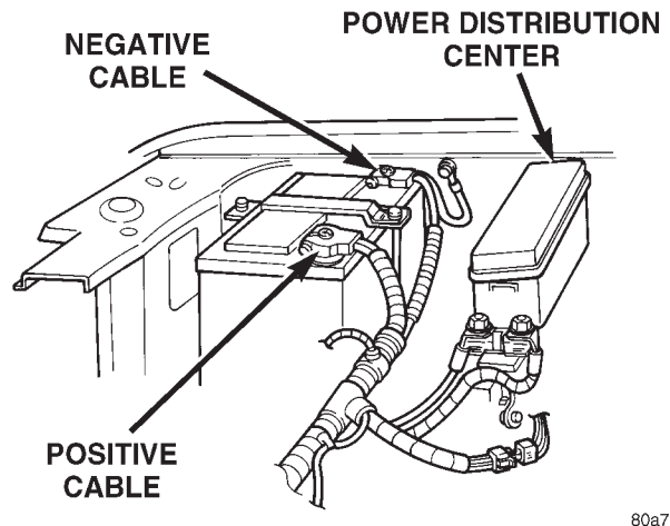
Fig. 21 Battery Cables
